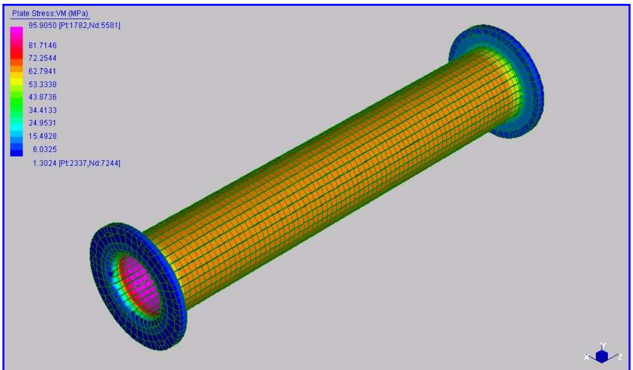
A composite hydraulic ram analysis
